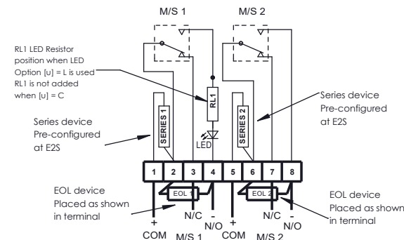
Circuit shown in Unoperated condition
