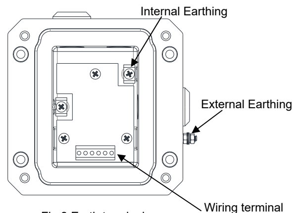
Fig 3 Earth terminals
