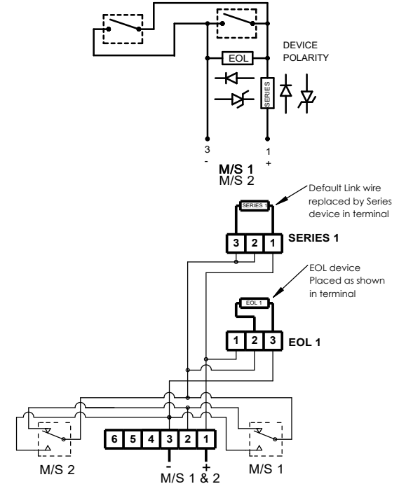
Circuit as shown in Unoperated condition
