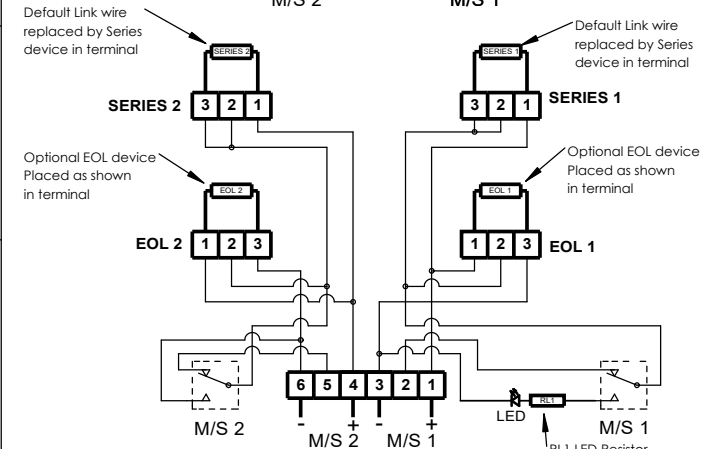
Circuit as shown in Unoperated condition
