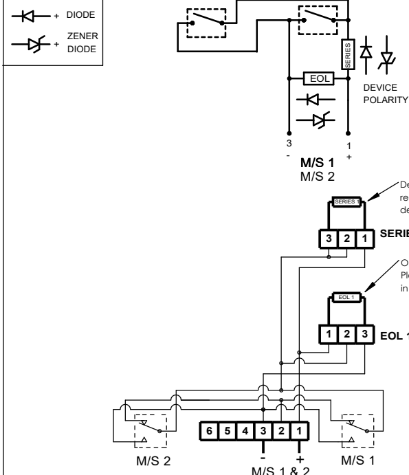
Circuit as shown in Unoperated condition
