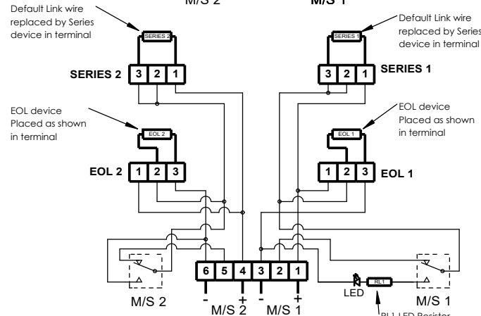
Circuit as shown in Unoperated condition
