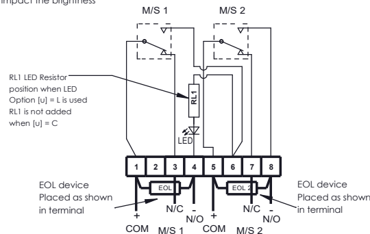
Circuit shown in Unoperated condition
