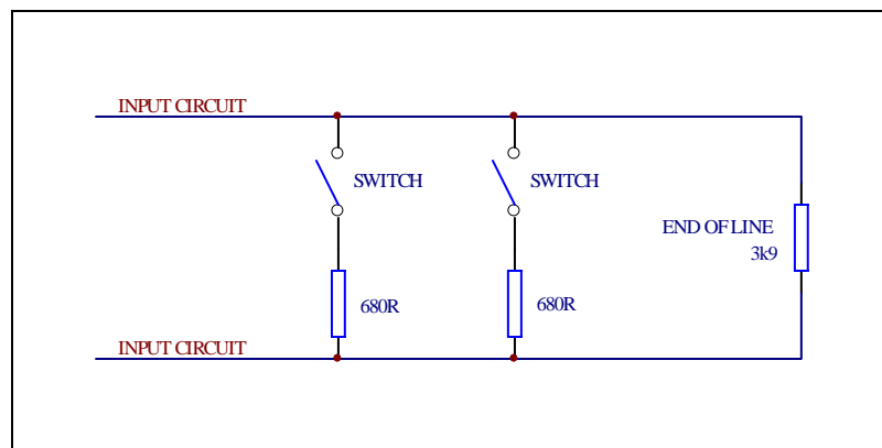
Figure 1 – Input circuit configuration
