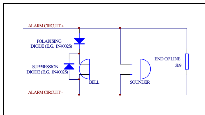
Figure 2 – Alarm circuit configuration
